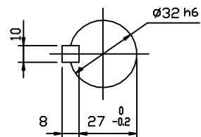
OUTPUT SHAFT
